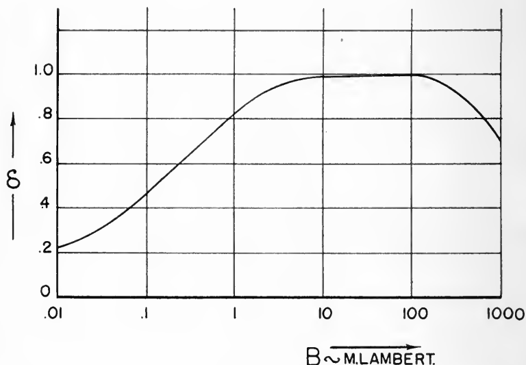
FIG. 12. \delta - B diagram: The discrimination factor \delta is plotted against the absolute brightness. The scale for \delta is shown arbitrarily so that \delta = 1 for the brightness region in which Fechner's law is valid.
